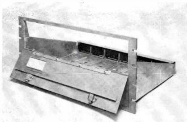
FIG. 4. BR-2A Shelf has front panel 8 \frac{3}{4} " high—is designed to mount on old-type open racks or new RCA cabinet racks.
