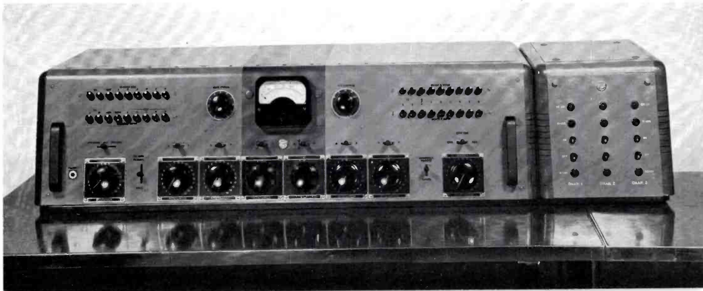
FIG. 5. The 76-B4 Console (left) with a BCS-1A Sub-control Console. In this system one such unit is located in each control room. "Ready" switches on the master unit allow switching function to be performed at the sub-control unit when desirable
