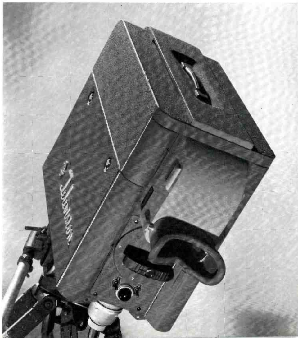
(Left) Side view of the RCA Type TK-30A Field Camera which uses the Image Orthicon tube.
