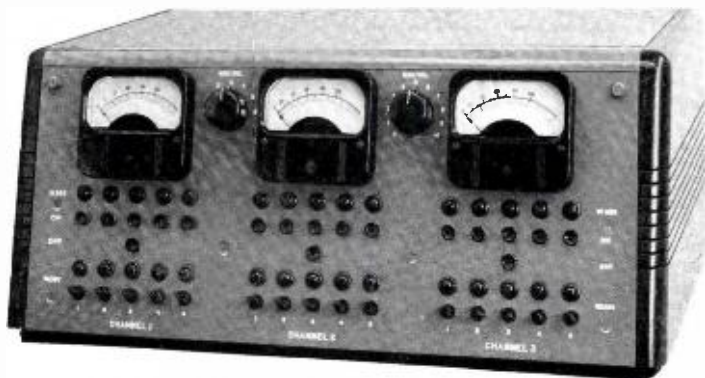
FIG. 7. (Left) Closeup of Master Console. Controls under each meter (from top to bottom) are: five "In use" lights, five "On" push-buttons, one "Off" push-button, five "Ready" lights, and five "Ready" switches.
