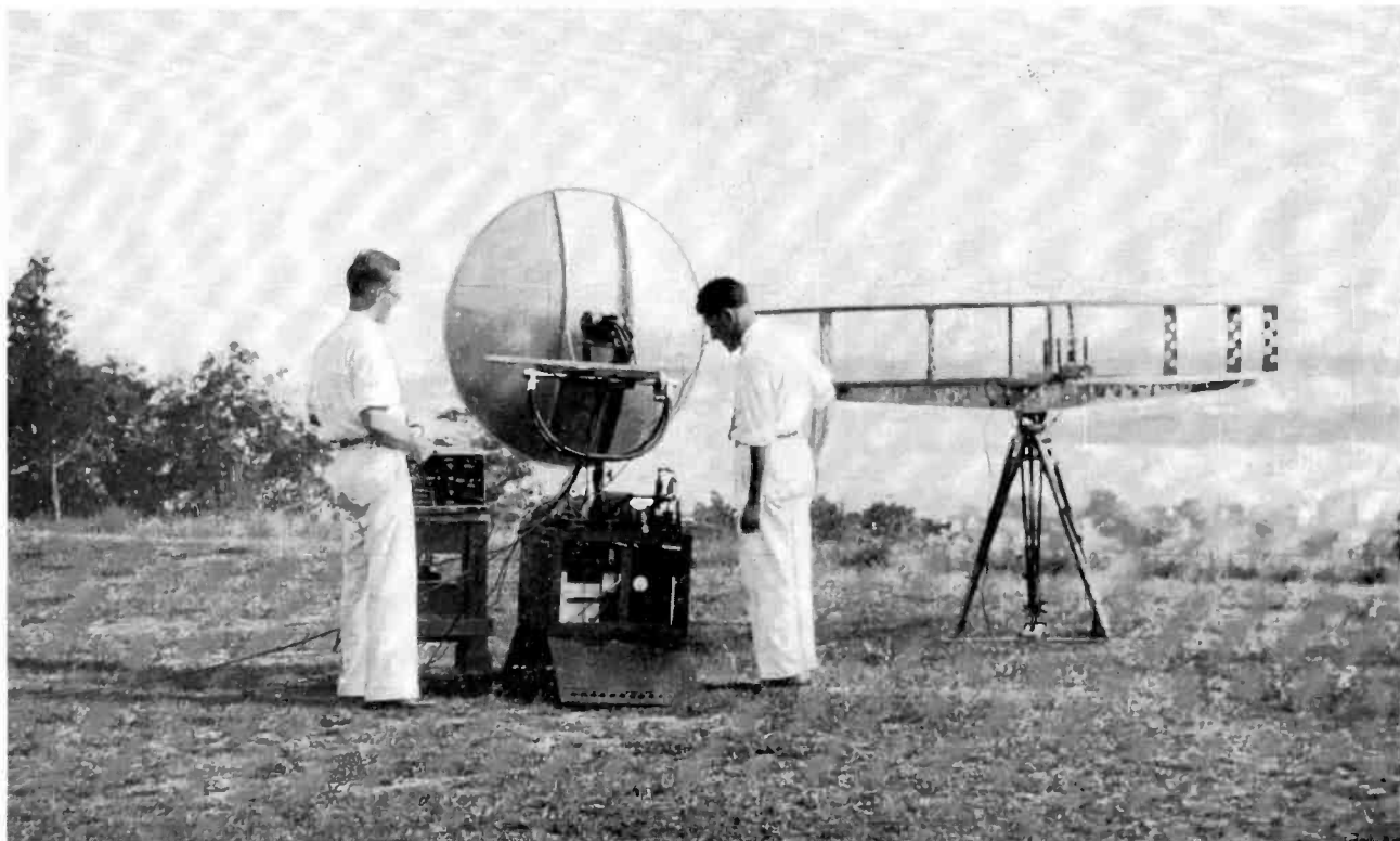
FIG. 4. RCA engineers pioneered in the development of microwave equipment for radar and communications purposes. The illustration above shows Dr. E. G. Linder and Dr. Irving Wolfe, of RCA Laboratories, with a voice-modulated 9 cm. transmitter set up at Navisink Light in the summer of 1934. The equipment to the right is a Signal Corps 60 cm. transmitter
