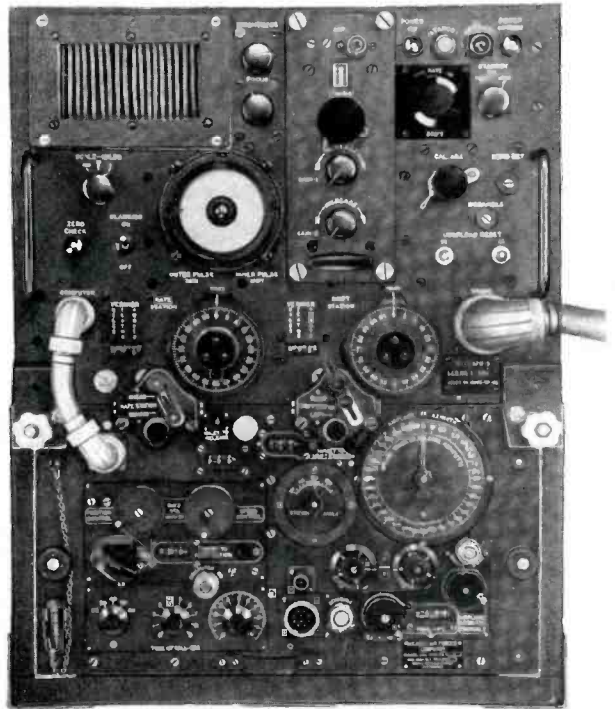
FIG. 12. SHORAN—This is the airborne part of the fantastically accurate bombing equipment known as SHORAN. Developed by RCA, this system has been described by the AAF as the most accurate of all bombing methods. It is now being used by map makers, oil geologists and others as a precision surveying instrument.
