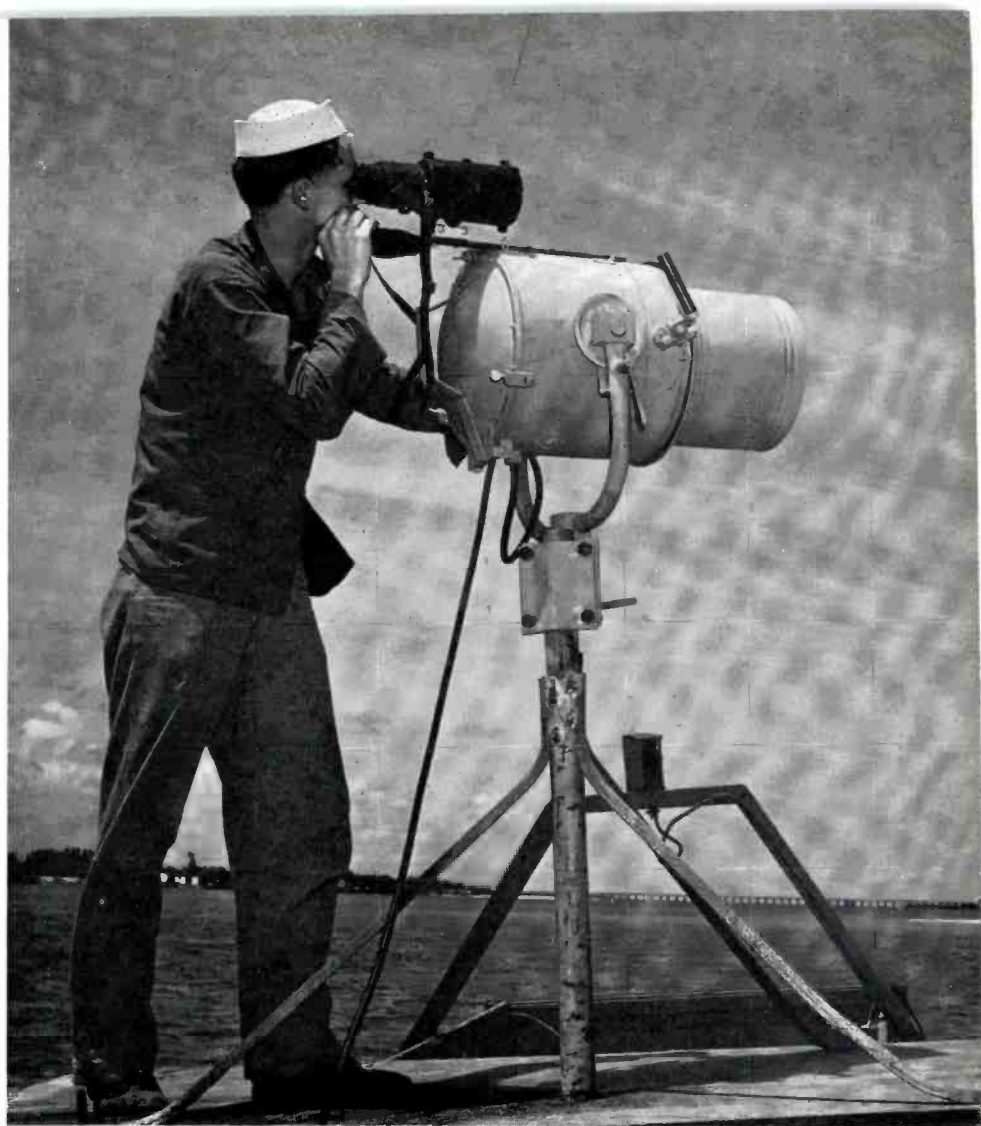
FIG. 2. INFRARED TELESCOPE —This instrument, using a very sensitive image tube in conjunction with an infrared searchlight, is able to pick up (in total darkness) a shoreline a mile away or identify trucks and tanks at 700 feet. The infrared devices shown on this page are only a few of the numerous types developed by RCA engineers.
