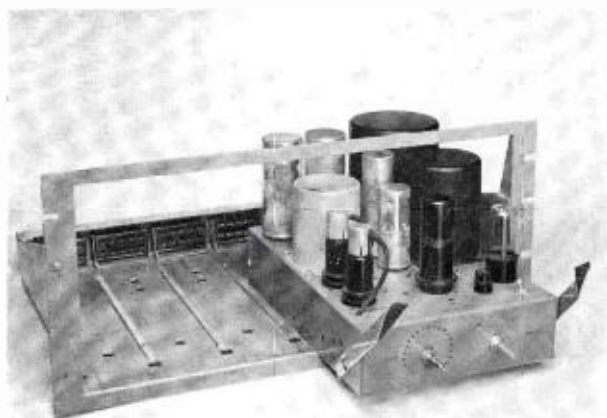
FIG. 6. With front panel of BR-2A removed, amplifiers easily slide into place. Guide strips on shelf insure proper positioning.
