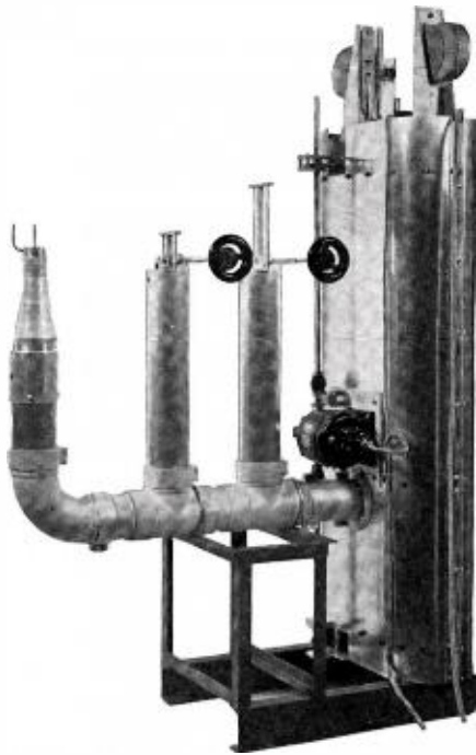
FIG. 10. MILLION WATT OSCILLATOR —This is an external view of an oscillator which uses two A-2231's to provide an output of 1,000,000 watts duty cycle 0.1 per cent at 600 megacycles. Note directional antenna on the end of the transmission line.
