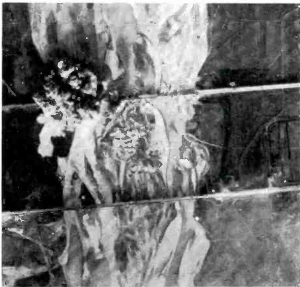
FIG. 13. SHORAN BOMBING—Photo at left shows cluster of bursts from bombs dropped by SHORAN direction on a railroad bridge in Italy. Earlier visual bombing (note old bomb pocks) had failed to destroy this bridge. SHORAN bombing cut four spans as evidenced by photo at right (note lack of shadows for these spans).
