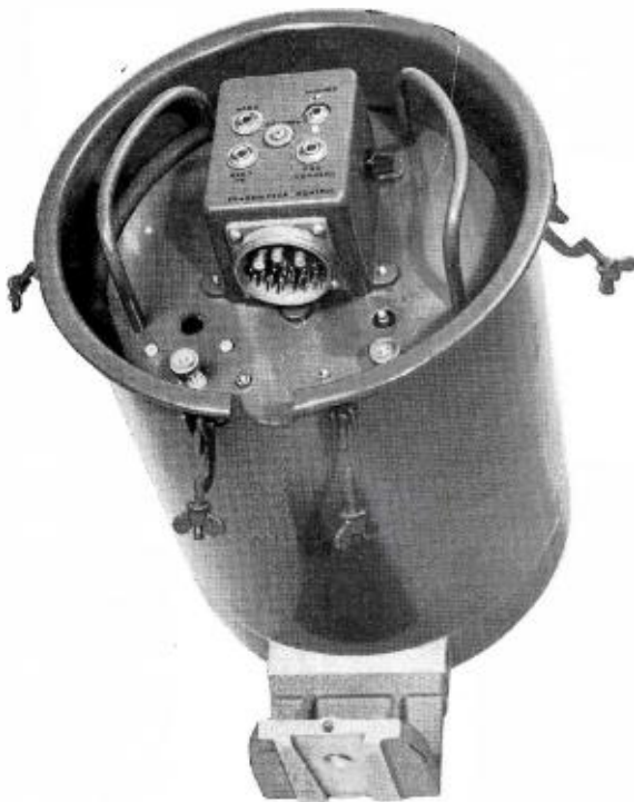
FIG. 9. When the weather-proof back cover is removed, the cable connection (center) and metering jacks are accessible. Cable, which is similar to standard camera cables, allows transmitter control to be located 400 feet away.
