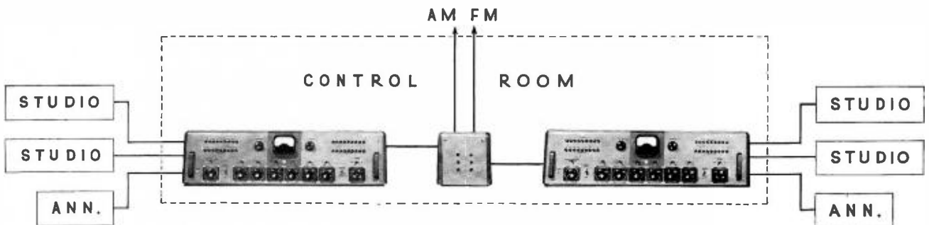
FIG. 3b. This is an alternative arrangement which may be used where both consolets are located in a single control room. Consolets may handle from one to three studios each.
