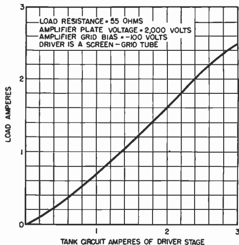
FIG. 6. Class-B power amplification characteristic of grounded-grid circuit.
