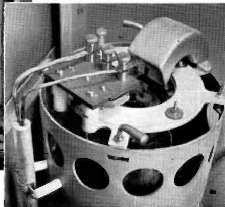
Amplifier tank assembly (right half of unit at left)—Visible are outer conductor of concentric-line plate tank, cathode transmission line at left, and motors to adjust cathode line, plate tank, and output coupling loop. Close-up below shows the RCA-7C24 in position, grid and filament clamps and connections, and air scoop to cool the tube seals.
